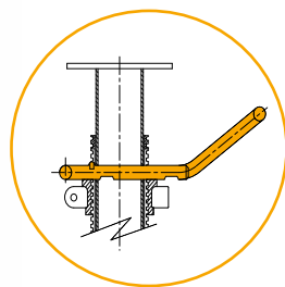
Cotter pin in working position
